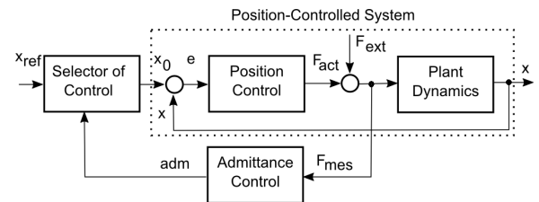
Fig. 2. Block scheme of a structure to control a robot joint with admittance control (inspired by [16])
