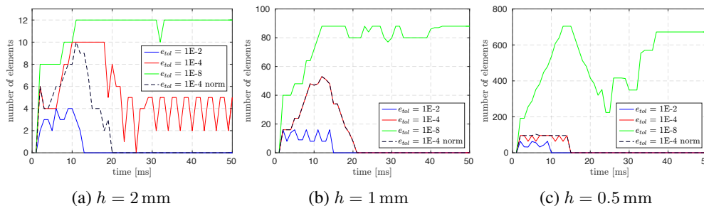
Figure 12. Number of elements with polynomial order of p = 10 during a p-adaptive simulation plotted over time for different element sizes h = 2, 1 and 0.5 mm until a time of 50 ms.
