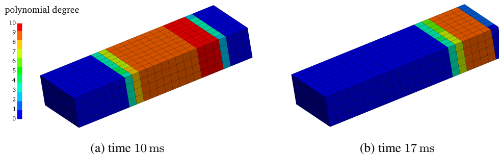
Figure 13. Polynomial degree distribution for two different time steps for a mesh with element size of 0.5 mm and a normalized error indicator.
