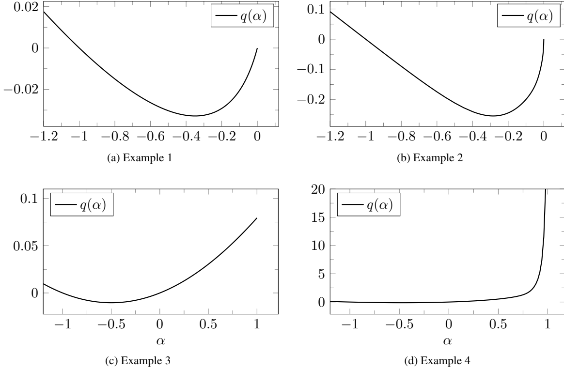
Figure 3: Entropic pressure for Examples 1-4. The lines are interrupted where q(\alpha) jumps to +\infty .
