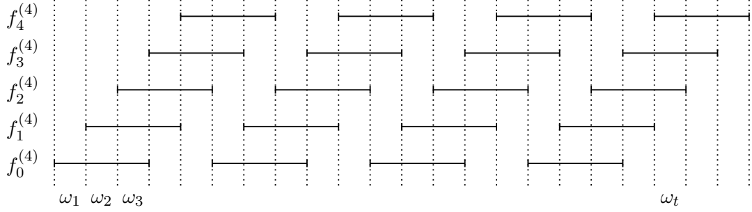
Figure 1: Illustration of (6.11) in the case n = 3 , \tau_n = 2 , M = 4
