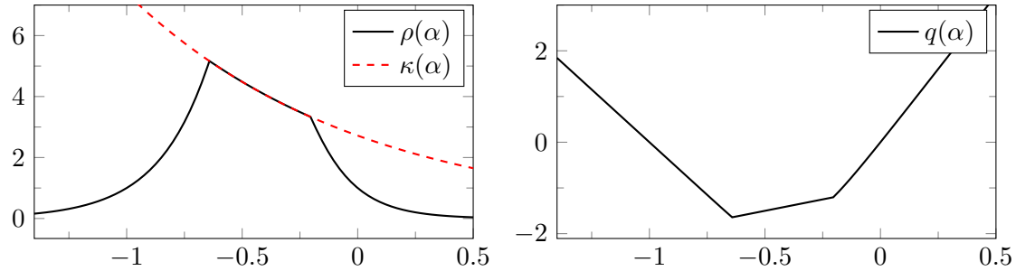
Figure 5: Entropic pressure and \rho(\alpha) in Example 6.
