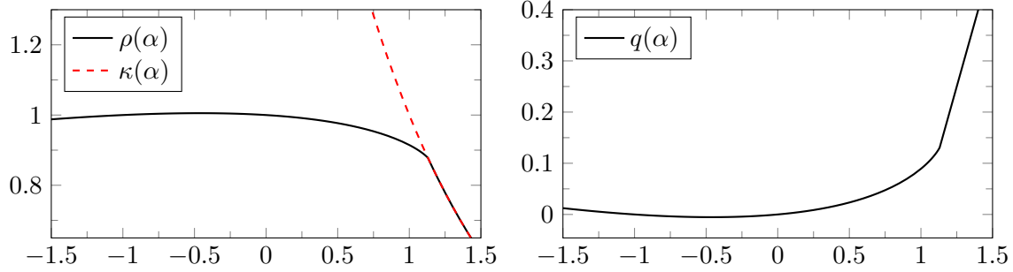
Figure 4: Entropic pressure and \rho(\alpha) in Example 5.
