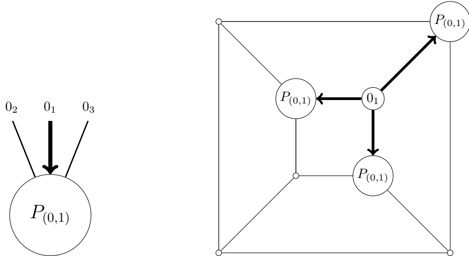
(a) The graph P_{(0,1)} . The arc (0,1) is the thick one.
