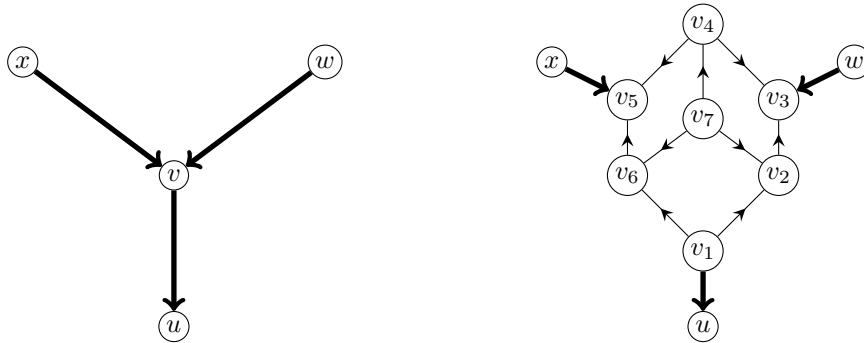
Figure 1: The replacement of R_v of a vertex v of graph D to obtain D' . The bold arcs are the arcs which are preserved (suspension arcs).
