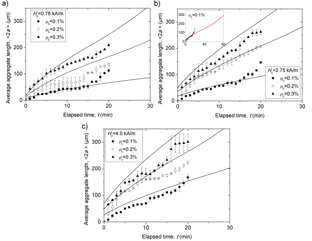
Fig. 9. Experimental and theoretical dependences of the average aggregate length on the elapsed time for different initial particle concentrations \varphi_0 and different magnetic field intensities H_0=0.78 kA/m (a); 2.75 kA/m (b); 4.0 kA/m (c). Symbols stand for the experiments, solid lines – for the theory. The inset in (b) shows the same dependency for \varphi_0=0.1\% in extended time scale. The experimental results were fitted by the theoretical dependences with the values of the adjustable parameters: \Theta = 3.3 \times 10^{-4} and \mathcal{G} = 5.0 \times 10^{12} .
