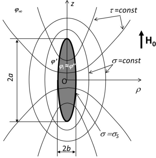
Fig.1. Sketch of the ellipsoidal aggregate. Cylindrical and ellipsoidal coordinates are introduced. Key values of the particle concentration inside the aggregate ( \varphi_i ), on the outer side of the aggregate surface ( \varphi' ) and far from the aggregate ( \varphi_\infty ) are also indicated. The external uniform magnetic field \mathbf{H}_0 is oriented along the z-axis.
