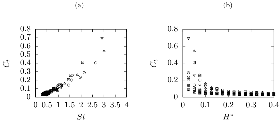
FIGURE 11. Thrust coefficient C_t as a function of (a) the Strouhal number St and (b) aspect ratio H^* . Different symbols correspond to different actuations: heaving ( \square ), pitching ( \circ ) and combined heaving and pitching at \phi = 0 ( \triangle ) and \phi = -\pi/2 ( \nabla )
