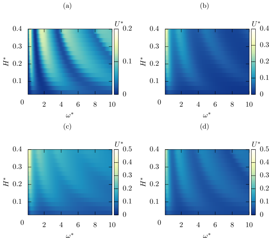
FIGURE 6. Cruising speed U^* predicted by the numerical model as a function of the non-dimensional flapping frequency \omega^* and the plate aspect ratio H^* for (a) pure heave, (b) pure pitch, (c) pitch and heave with zero phase lag, i.e. \phi = 0 , and (d) pitch and heave with \phi = -\pi/2 .
