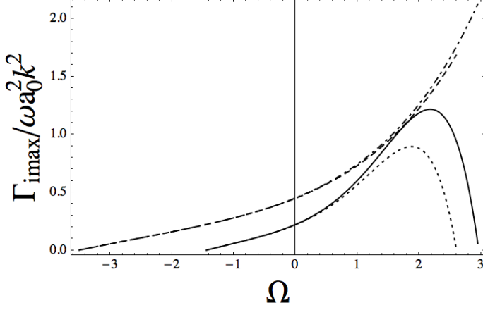
FIGURE 2. Dimensionless maximal growth rate of modulational instability as a function of \Omega in finite depth ( \mu = 2 ) and deep water ( \mu = \infty ). Solid line ( \kappa = 0.005 , \mu = 2 ); Dot-dashed line ( \kappa = 0.005 , \mu = \infty ); Dotted line ( \kappa = 0 , \mu = 2 ); Dashed line ( \kappa = 0 , \mu = \infty )
