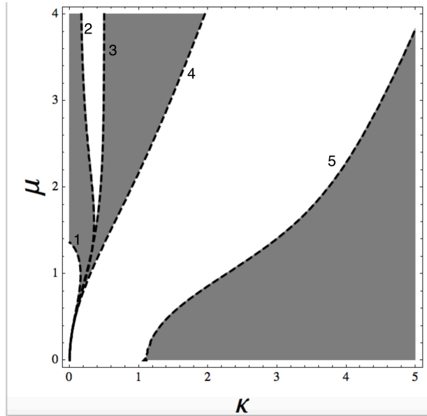
FIGURE 5. (\mu, \kappa) -instability diagram for gravity-capillary waves, matching the results from Djordjevic & Redekopp (1977) (dashed lines). Here, there is no vorticity. The unstable regions are in gray whereas stable regions are in white.
