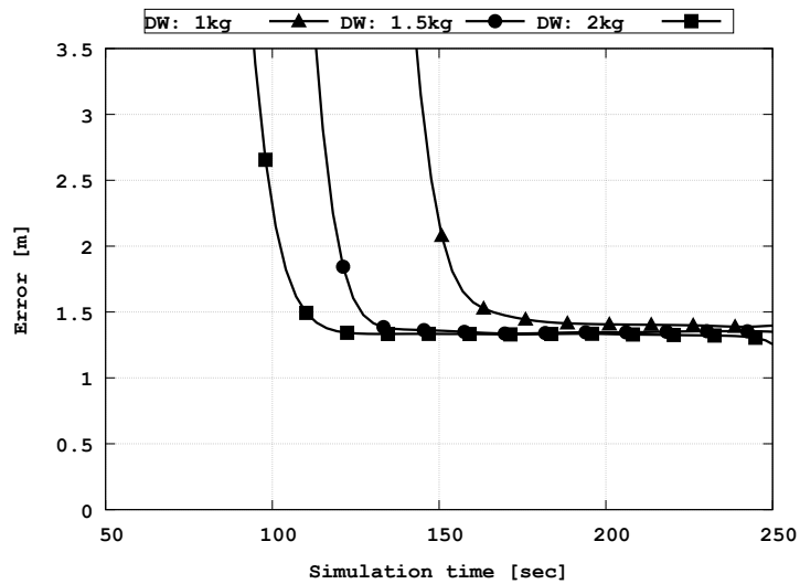
Figure 13: Evolution of the average formation error with a varying drone weight and \gamma = 80
