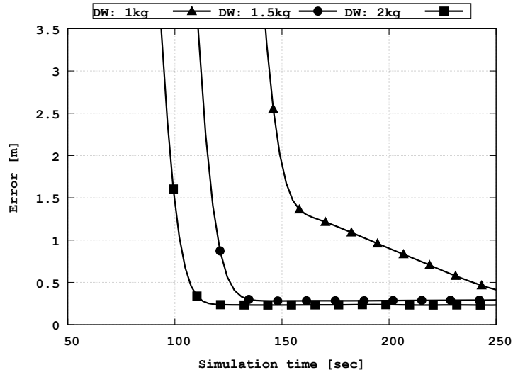
Figure 11: Evolution of the average formation error with a varying drone weight and \gamma = 0
