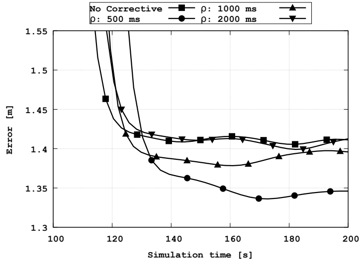
Figure 10: Evolution of the average formation error with a varying \rho and \gamma = 70
