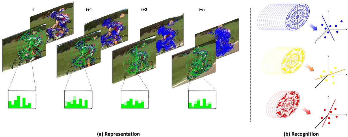
Figure 1: Pipeline of the proposed approach: (a) spatio-temporal representation of the proposed motion descriptor. First, a set of point trajectories are computed from the video. Then, a polar representation is centered in each frame around the potential action defined by the end points of the active trajectories. A histogram is computed in each polar region to estimate the partial distribution of kinematics. The histograms are updated at each time by considering different time intervals, thus enabling frame-level recognition. (b) recognition process using the SVM. Different histogram versions are built at each time corresponding to different time depth. Each one of these action descriptors is mapped to its respective SVM and a recognition label is returned at each frame.
