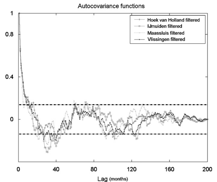
Fig. 7. ACFs of monthly SLH records filtered by the EOFs. The band delimited by the two horizontal lines indicates the 95% confidence interval.
