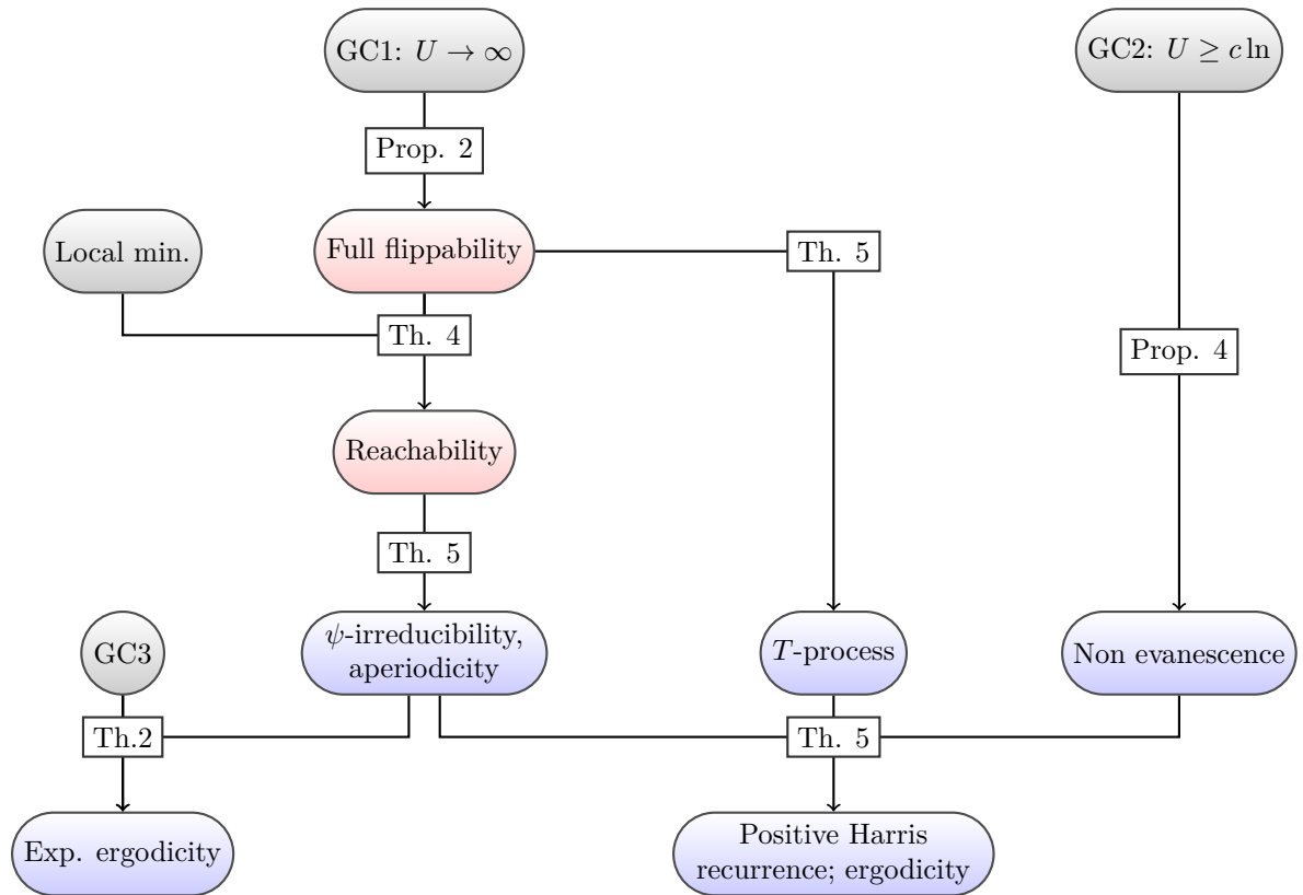
Schematic overview of key properties of the zigzag process in relation to the Growth Conditions 1, 2 and 3. The grey nodes represent conditions on the potential U , the red nodes refer to deterministic ‘reachability’ properties of trajectories, discussed in Section 2, and the blue nodes represent probabilistic properties discussed in Section 3.
