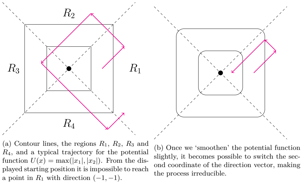
Figure 1: The canonical zigzag process for U(x) = \max(|x_1|, |x_2|) and a smoothed version of U .
