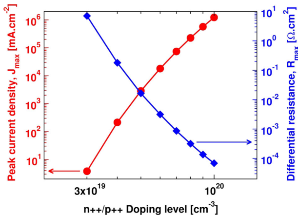
Fig. 5 Characteristic of the tunnel junction as a function of the doping level. The peak current density J_{\max} ( \text{mA cm}^{-2} ) and the differential resistance R_{\max} ( \Omega \text{ cm}^2 ) are marked by red circles and blue squares, respectively. (Color figure online)
