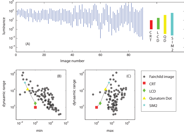
Figure 1. (A) The luminance range of images for the Fairchild high dynamic range survey and various monitor types. The images are sorted from lowest dynamic range and various monitor types. (B) Scatter plot of the minimum luminance against dynamic range (C) Scatter plot of the maximum luminance against dynamic range.
