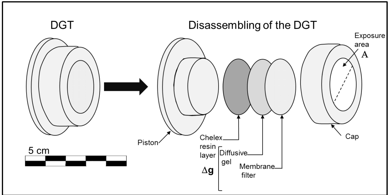
Figure 1: Schematic representation of DGT unit assembled and disassembled, A is the exposure surface area of the membrane, Δg is the thickness of the diffusion layer (diffusive gel + filter membrane).
