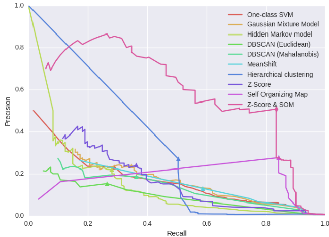
Figure 4. Precision-recall curves
