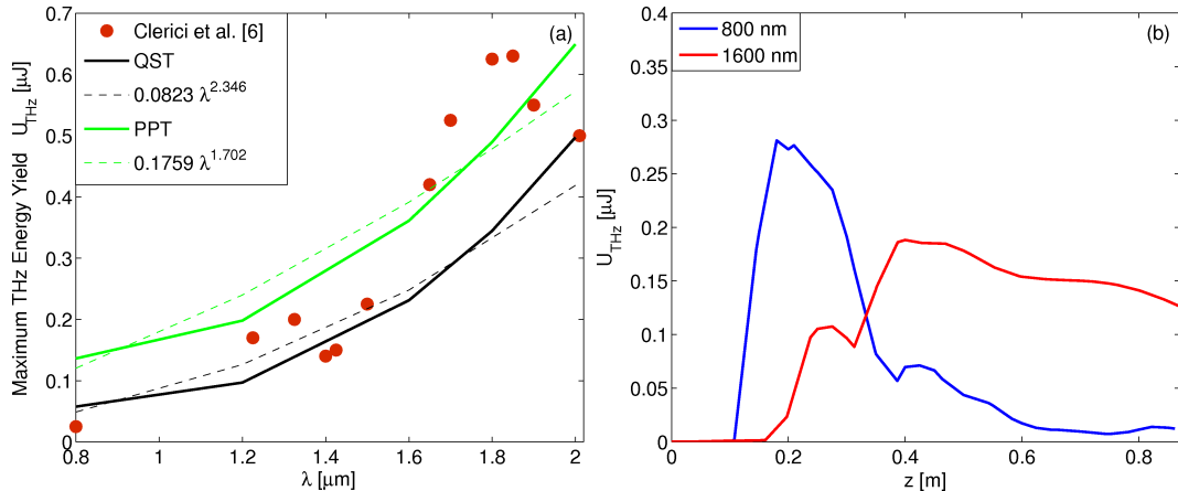
Figure 1 (a) 3D simulation results of THz yields computed from a unidirectional pulse propagator for focused two-color 60-fs Gaussian pulses with a quasi-static ionization model (black curves) or the Perelomov-Popov-Terent'ev ionization rate (green curves) for air molecules. Maximum THz energy yield ( \nu \leq 80 THz) as a function of the pump wavelength and corresponding scaling curves in \lambda^\alpha (dashed curves). The red dots recall the experimental data points of [6]. (b) THz energy in a 80-THz frequency window of two-color 40-fs filaments simulated for 800-nm (blue curves) and 1600-nm (red curves) pump pulses.
