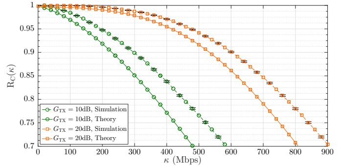
Fig. 6. Rate coverage probability R_{\text{C}} as a function of the threshold \kappa , for \alpha_{\text{N}} = 4 , \psi = 30^\circ , G_{\text{TX}} = \{10 \text{ dB}, 20 \text{ dB}\} , \lambda_{\text{BS}} = 4 \cdot 10^{-3} , N_o = 2 .
