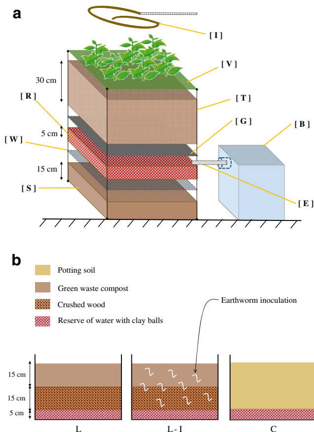
Fig. 2 a Schematic drawing of experimental box. Legend: [B] bottle storage for the overflow of water, [E] evacuation, [G] geotextile, [I] drip irrigation system, [R] reserve of water with clay balls, [S] wooden pieces to raise the box, [T] Technosol, [V] vegetation layer, and [W] waterproof membrane. b Description of the three treatments of the experiment
