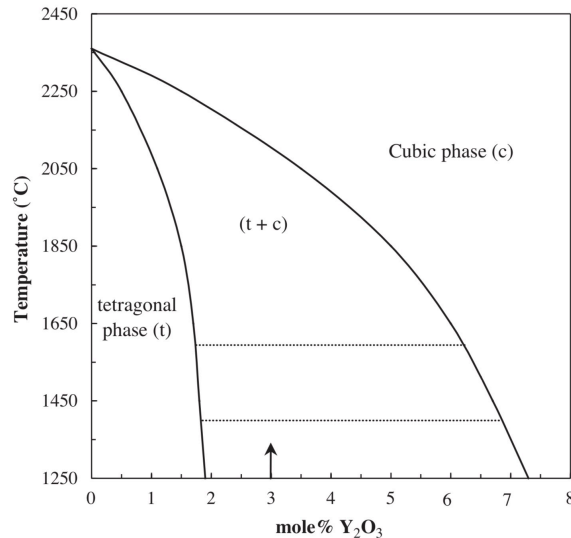
Fig. 1. Selected region of the \text{ZrO}_2\text{-Y}_2\text{O}_3 equilibrium phase diagram (after Scott [15]). The dashed lines show the typical range of sintering temperatures of 3 mol % yttria-stabilized zirconia.
