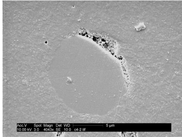
Fig. 7. Scanning electron micrograph of a 3Y-TZP ceramic sintered at 1550°C for 5 h, after 24 h aging at 134°C.
