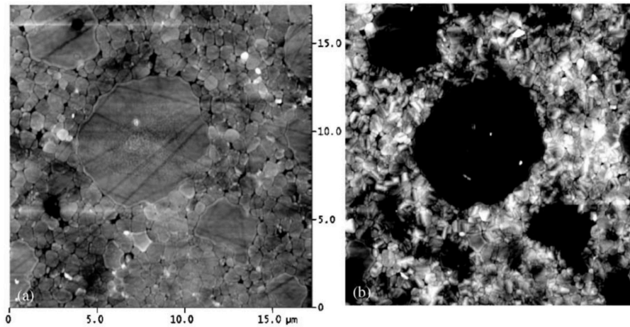
Fig. 5. Atomic force microscopy images of the same zone, (a) before and (b) after 24 h aging at 134°C, for a 3Y-TZP ceramic sintered at 1550°C for 5 h.
