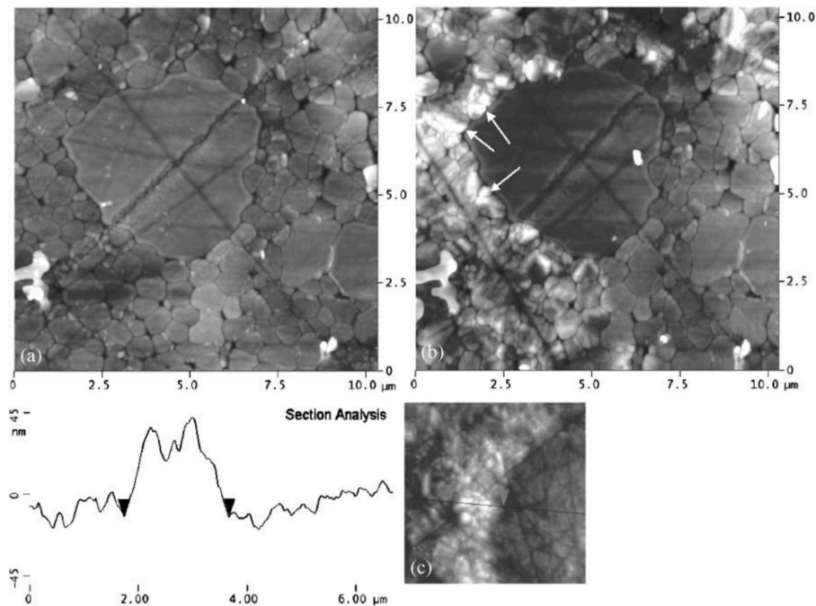
Fig. 4. Atomic force microscopy images of the same zone, (a) before and (b) after 1 h aging at 134°C, for a 3Y–TZP ceramic sintered at 1550°C for 5 h. Arrows indicate surface uplifts due to the t–m transformation of tetragonal grains. (c) Corresponds to a line scan at the periphery of a cubic grains after 1 h aging.
