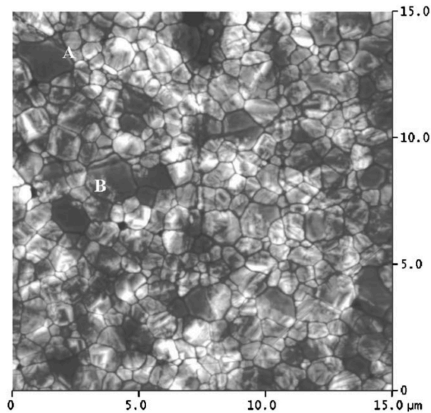
Fig. 6. Atomic force microscopy images of a 3Y-TZP ceramic sintered at 1450°C for 5 h, after 24 h aging at 134°C.
