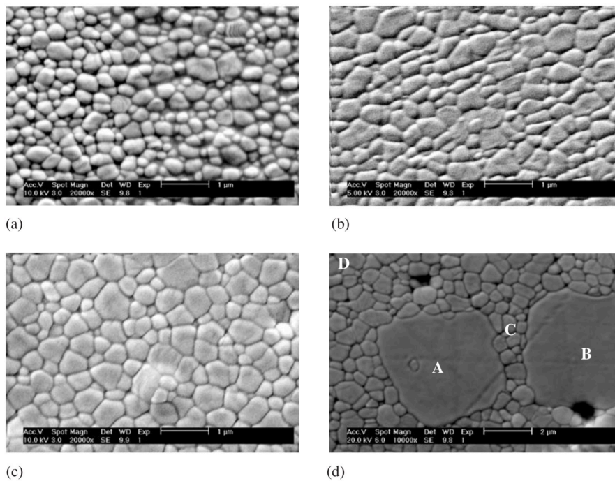
Fig. 2. Scanning electron microscopy images of 3 mol % Y-TZP ceramics: (a) sintered at 1450°C for 2 h, (b) sintered at 1450°C for 5 h, (c) sintered at 1550°C for 2 h, (d) sintered at 1550°C for 5 h. Points denoted from A to D are regions where EDS spectra were performed.
