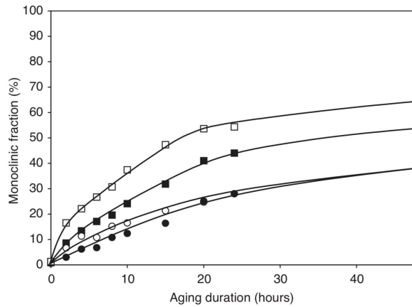
Fig. 3. Aging kinetics, at 134°C under 2-bars pressure, of 3 mol % Y-TZP ceramics: (●) sintered at 1450°C for 2 h, (○) sintered at 1450°C for 5 h, (■) sintered at 1550°C for 2 h, (□) sintered at 1550°C for 5 h.
