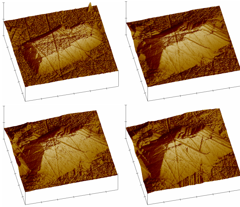
Fig. 1a: Observation of partial transformation and internal growth. Ageing steps of 20 hrs. Horizontal scale: 1 \mu\text{m}/\text{div} , vertical scale: 250 nm/div.
