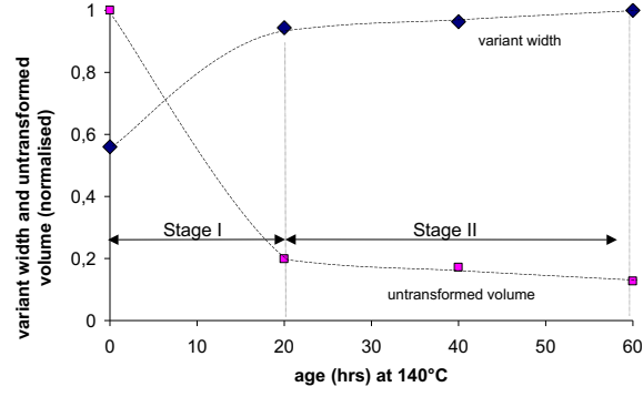
Fig. 4: Normalised variant width as a function of its age, internal growth mode.
