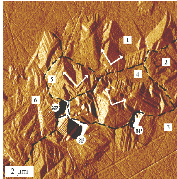
Fig. 10: Observation of transformation induced relief in a large portion of the surface. The relief features allow the approximate determination of the location of grain boundaries. Deduced grains are numbered, and grain pop-out (gp) locations are indicated. Grains 1, 4 and 5 present a very low crystallographic disorientation. Dashed lines represent the expected grain boundaries.
