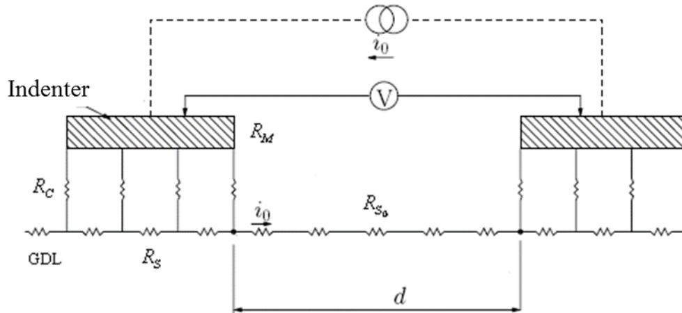
Fig. 6. Description of the different resistances involved in the TLM method.
