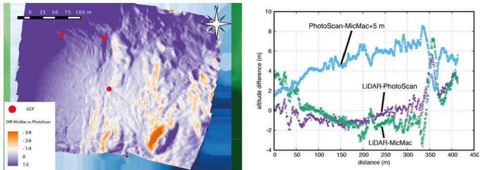
FIG. 6. Left: map of the DEM difference. The positioning mismatch is obvious in the lower-right corner where a hill exhibits a positive height difference on the right and negative height difference on the left. Right: cross section of DEM differences between the airborne lidar dataset and two DEMs generated from photogrammetric processing of the same pictures with the same camera GNSS coordinates provided in each picture Exif header, using Agisoft PhotoScan and MicMac. So that the graph is readable, +5 m was added to the PhotoScan–MicMac difference.
