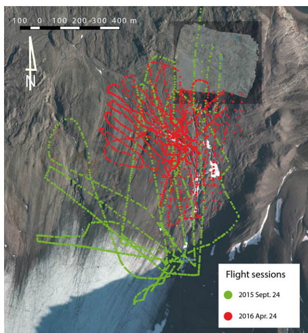
FIG. 3. Two manual flight paths for September 2015 and April 2016. The dots represent the GNSS position of each acquired photograph over features of interest.
