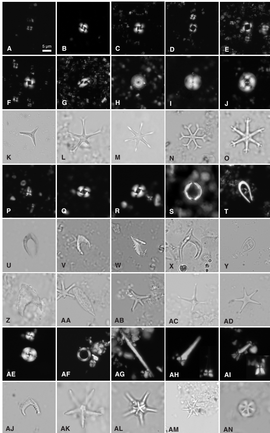
Figure F31. Calcareous nannofossils from selected Expedition 363 sites. A. Emiliania huxleyi ; U1485A-1H-CC. B. Gephyrocapsa oceanica ; U1485A-1H-CC. C. Gephyrocapsa >5.5 \mu\text{m} ; U1486B-8H-CC. D,E. Pseudoemiliania lacunosa ; (D) U1489C-2H-6, 60 cm, (E) U1489B-2H-6, 75 cm. F. Reticulofenestra asanoi ; U1483A-9H-6, 50 cm. G. Helicosphaera sellii ; U1486B-10H-CC. H, I. Calcidiscus macintyreii ; (H) U1486B-12H-CC, (I) U1486B-19H-CC. J. Coccolithus pelagicus ; U1486B-15H-CC. K. Discoaster triradiatus ; U1482A-18H-CC. L. Discoaster pentaradiatus ; U1489C-8H-4, 60 cm. M. Discoaster brouweri ; U1482A-12H-2, 75 cm. N. Discoaster variabilis ; U1489B-12H-CC. O. Discoaster surculus ; U1482B-38H-CC. P. Sphenolithus abies ; U1483A 31H-CC. Q, R. Reticulofenestra pseudoumbilicus ; (Q) U1483A-31H-CC, (R) U1489B-10H-CC. S. Scyphosphaera globulata ; U1488A-14H-2, 60 cm. T, U. Ceratolithus cristatus ; (T) U1489B-3H-CC, (U) U1428B-18H-CC. V, W. Ceratolithus armatus ; (V) U1482B-27H-4, 50 cm, (W) U1482B-27H-CC. X. Amaurolithus tricorniculatus ; U1482A-22H-6, 75 cm. Y. Amaurolithus delicatus ; U1482B-27H-CC. Z. Amaurolithus primus ; U1489C-22H-CC. AA. Triquetrorhabdulus carinatus ; U1489C-31F-CC. AB. Discoaster sp.; U1486B-22H-6, 81 cm. AC. Discoaster tamalis ; U1489B-6H-CC. AD. Discoaster asymmetricus ; U1483A-31H-CC. AE. Cyclicargolithus floridanus ; U1489C-38X-6, 40 cm. AF. Coronocyclus nitescens ; U1489C-42X-4, 30 cm. AG. Triquetrorhabdulus carinatus ; U1489C-41X-CC. AH. Sphenolithus heteromorphus ; U1489C-41X-CC. AI. Sphenolithus belemnus ; U1489C-41X-CC. AJ. Nicklithus amplificus ; U1482B-33H-CC. AK. Discoaster quinquerramus ; U1489C-24H-CC. AL. Discoaster berggrenii ; 1482C-41X-CC. AM. Catinaster calyculus ; U1489C-31F-CC. AN. Catinaster coalitus ; U1489C-30F-CC.
