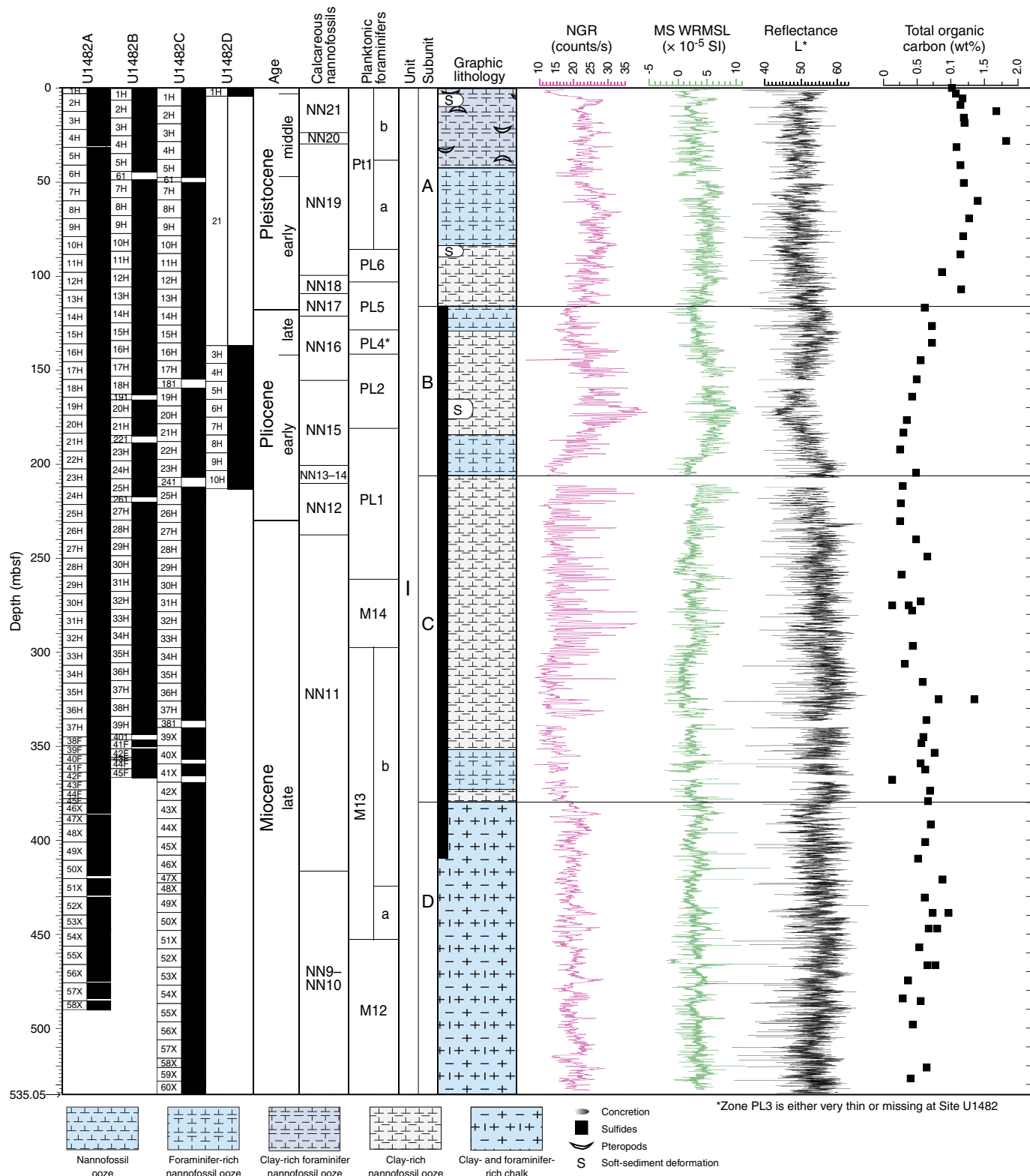
Figure F8. Summary of Site U1482 results. NGR = natural gamma radiation, MS = magnetic susceptibility, WRMSL = Whole-Round Multisensor Logger.
