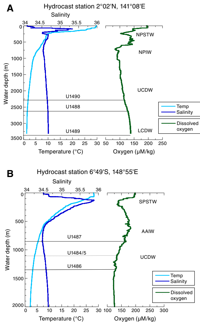
Figure F5. Hydrographic profiles from (A) the southern Eauripik Rise (B) northeast Papua New Guinea. NPSTW=North Pacific Subtropical Water, SPSTW=South Pacific Subtropical Water, NPIW= North Pacific Intermediate Water, AAIW= Antarctic Intermediate Water, UCDW= Upper Circumpolar Deep Water, LCDW= Lower Circumpolar Deep Water. From Y. Rosenthal (unpubl. data).
