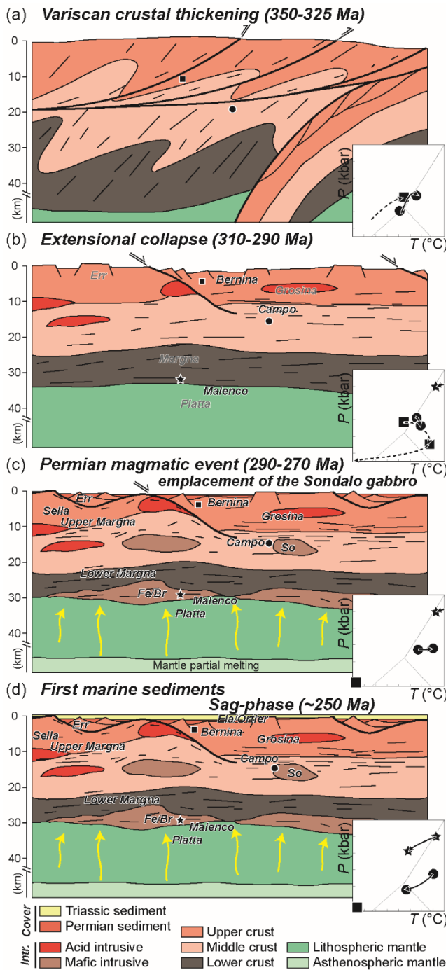
Fig. 9: Schematic tectonic evolution of the Austroalpine domain during (a) Variscan orogeny (350–325 Ma), (b) Extensional collapse of the Variscan orogeny (310–290 Ma), (c) the Permian magmatic event (290–270 Ma) and (d) post-tectonic cooling of the lithosphere. See text for detailed explanations. “Fe”, “Br” and “So” refer to the Fedoz, the Braccia and the Sondalo gabbro, respectively. P - T data are compiled from Spillmann and Büchi (1993), Müntener et al. (2000) and Petri et al. (2016). The position of different Austroalpine units is indicated (in transparency when poorly constrained)
