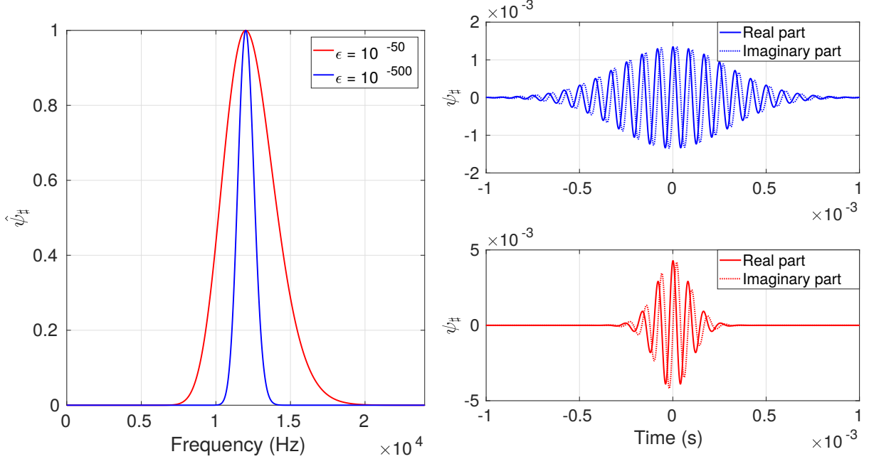
Fig. 1. Left: Fourier transform of the sharp wavelet \psi_\# for two different values of \epsilon . Right: Corresponding wavelets in the time domain: \epsilon = 10^{-500} (top) and \epsilon = 10^{-50} (bottom). Here, \nu_0 = F_s/4 = 11025 Hz and \nu_1 = F_s/2 = 22050 Hz.
