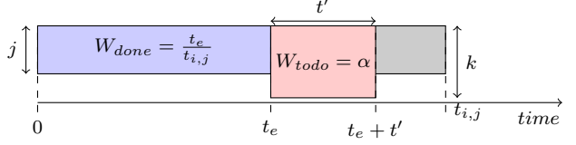
Figure 2: Work representation for application T_i at time t_e .
