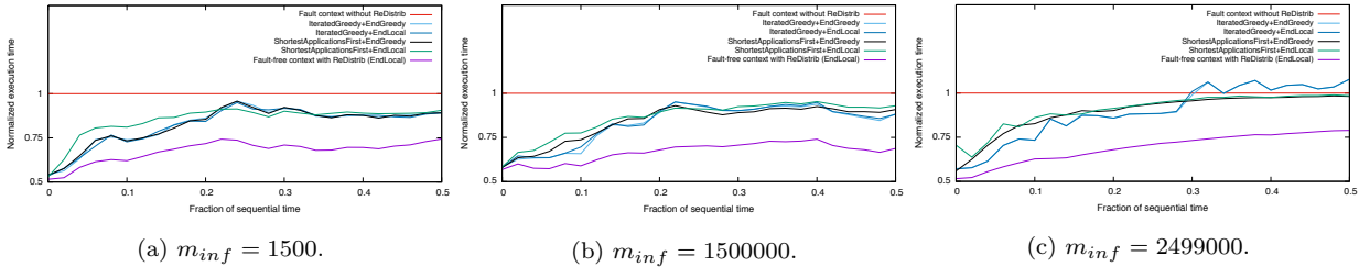
Figure 16: Impact of the sequential fraction of time with n = 100 and p = 1000 when 0 \leq f \leq 0.5 .
