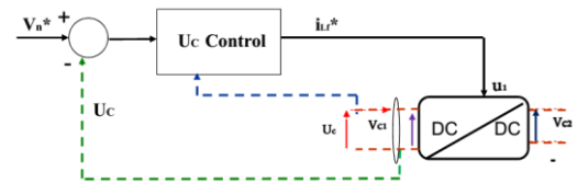
Figure: 3 DC/DC Buck
