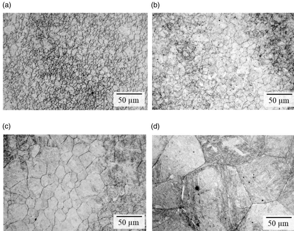
Figure 5. Different chosen grain size steels for RCF tests: (a) G_{ASTM} = 10 , Mean grain diameter = 11 \mu\text{m} , T_{A4} = 900^\circ\text{C} ; (b) G_{ASTM} = 8 , Mean grain diameter = 20 \mu\text{m} , T_{A3} = 975^\circ\text{C} ; (c) G_{ASTM} = 7 , Mean grain diameter = 30 \mu\text{m} , T_{A2} = 1000^\circ\text{C} ; (d) G_{ASTM} = 3 , Mean grain diameter = 120 \mu\text{m} , T_{A1} = 1100^\circ\text{C} .
