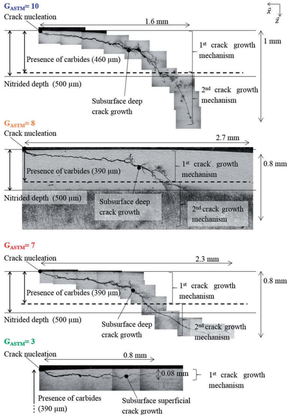
Figure 12. 2D crack morphologies on cross-sections at the contact centre of different nitrided microstructures. \vec{x} and \vec{z} correspond respectively to the rolling and depth directions.
