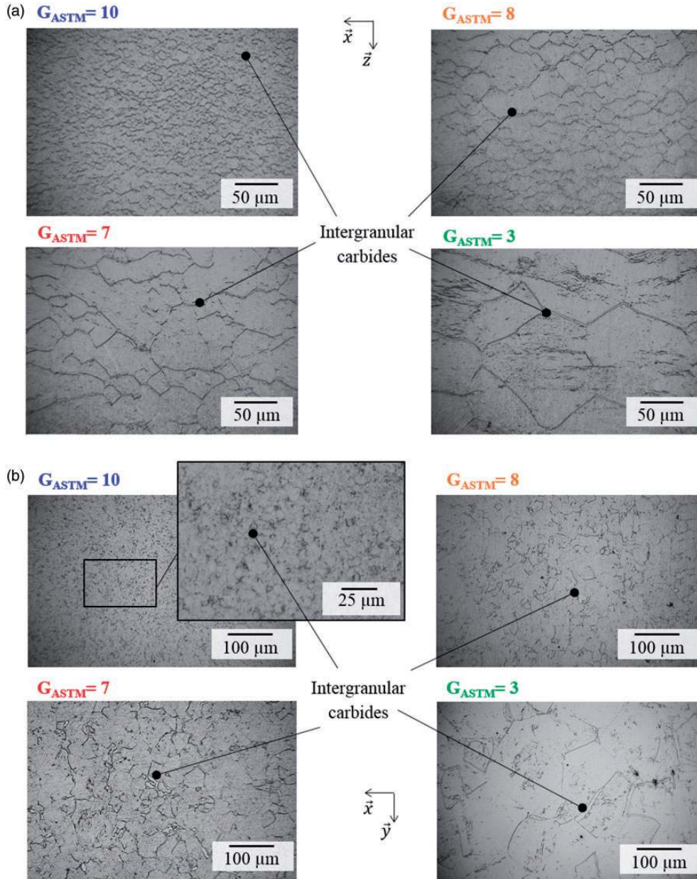
Figure 6. Different morphologies of intergranular carbides within the RCF tested nitrided microstructures (on cross-sections (a) perpendicular and (b) parallel to disc surfaces). \bar{x} and \bar{z} correspond respectively to the rolling and depth directions.
