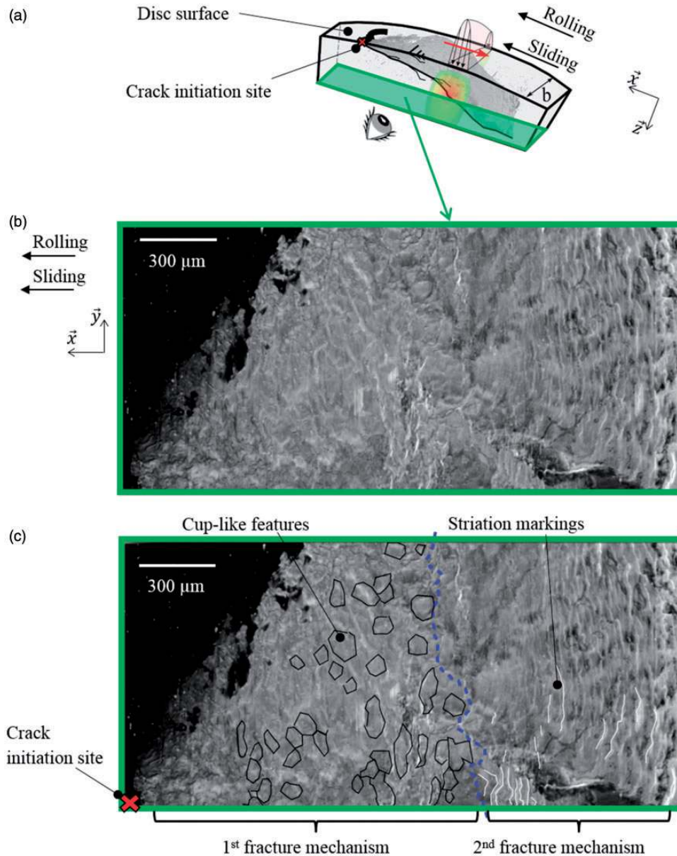
Figure 15. (a) Scheme of the sample analysed by X-ray tomography. (b) Resulting image of superposition of the 2D scanned images parallel to disc surface showing (c) the two fracture mechanisms. \bar{x} and \bar{z} correspond respectively to the rolling and depth directions.
