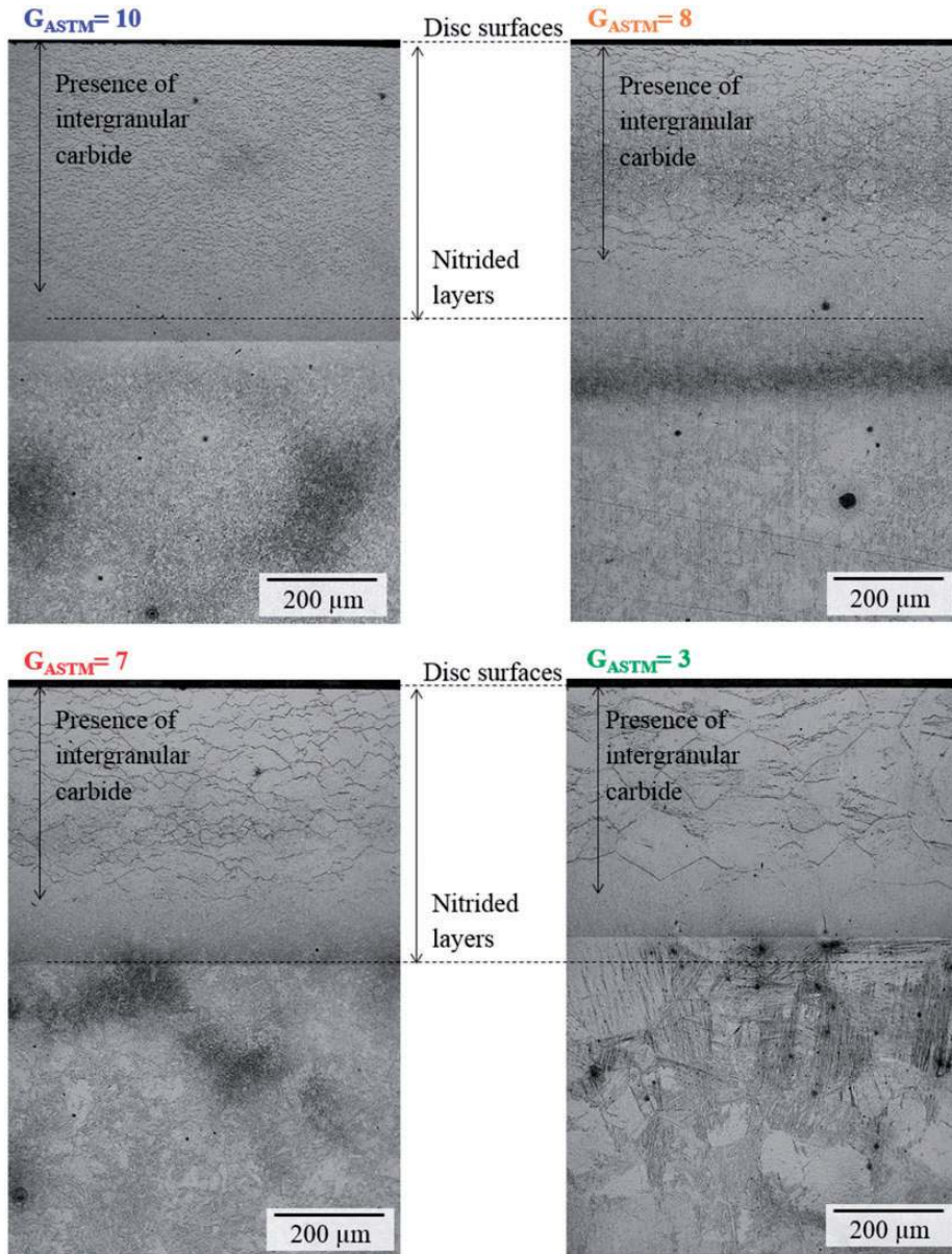
Figure 7. Cross-sections perpendicular to disc surfaces displaying the RCF tested nitrided microstructures.
