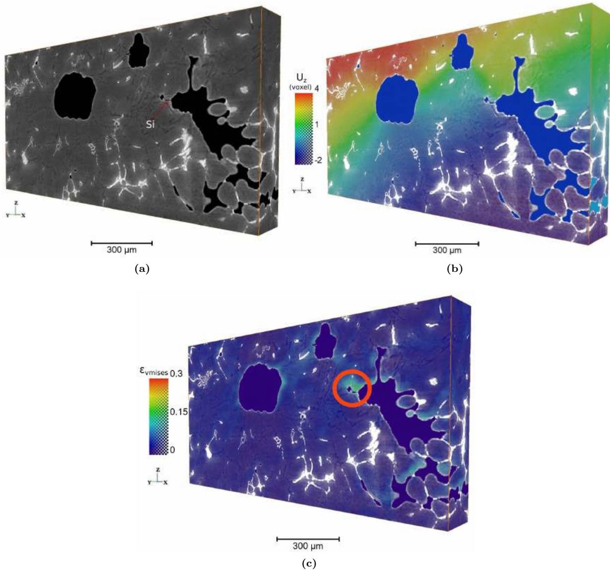
Figure 1: In situ low cycle fatigue testing of a cast Al alloy at T=250\text{ }^\circ\text{C} ; the uniaxial cyclic tensile load is vertical (a) 3D reconstruction of the complex microstructure of the alloy showing pores (in black) Si and intermetallic particles; the red arrow indicates a crack that has formed after one fatigue cycle on a Si particle (b) vertical displacement field in voxels (c) map of Von Mises strain showing strain localisation in the pore vicinity (scale bar in real values).
