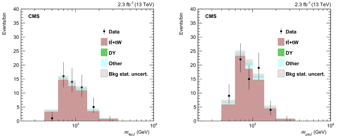
Fig. 3. Data events in the e\mu q\bar{q}' control regions used to estimate the \bar{t}\bar{t} + tW contribution in the eeq\bar{q}' (left) and \mu\mu q\bar{q}' (right) channels, compared to the expectations of the background simulations. “Other” stands for the contribution from W +jets and diboson events. (For interpretation of the references to colour in this figure, the reader is referred to the web version of this article.)
