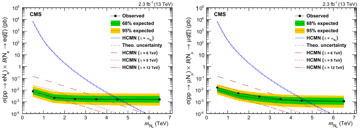
Fig. 5. The observed 95% CL upper limits (solid black lines) on \sigma(pp \rightarrow \ell N_\ell) \mathcal{B}(N_\ell \rightarrow \ell q\bar{q}') , obtained in the analysis of the ee\bar{q}\bar{q} (left) and the \mu\mu q\bar{q} (right) final states, as a function of the mass of the heavy composite Majorana neutrino, N_\ell . The corresponding expected limits are shown by the dotted lines, and the bands represent the expected variation of the limit to one and two standard deviation(s). The solid blue curve indicates the theoretical prediction of \sigma(pp \rightarrow \ell N_\ell) \mathcal{B}(N_\ell \rightarrow \ell q\bar{q}') for \Lambda = m_{N_\ell} . The uncertainty in the theoretical prediction is derived by taking into account the factorization and normalization scales. The light red textured curves give the theoretical predictions for three \Lambda values ranging from 6 to 12 TeV in steps of 3 TeV. (For interpretation of the references to colour in this figure legend, the reader is referred to the web version of this article.)
