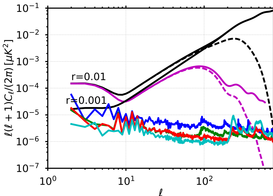
Figure 6. BB leakage power spectra for different scanning parameters. In cyan: \alpha = 65^\circ , \beta = 30^\circ , \tau_{\text{spin}}=10 min, \tau_{\text{prec}}=96.1803 min, red: \alpha = 50^\circ , \beta = 45^\circ , \tau_{\text{spin}}=10 min, \tau_{\text{prec}}=96.1803 min, green: \alpha = 50^\circ , \beta = 45^\circ , \tau_{\text{spin}}=2 min, \tau_{\text{prec}}=4 day, blue: \alpha = 30^\circ , \beta = 65^\circ , \tau_{\text{spin}}=2 min, \tau_{\text{prec}}=4 day. Spectra are computed for 222 detectors. Curves for the B mode model are described in the figure 4 caption. For the scanning strategies with a long precession period, we computed spectra for 100 detectors rescaling to 222 equivalent detectors using the 1/N_{\text{det}} dependence.
