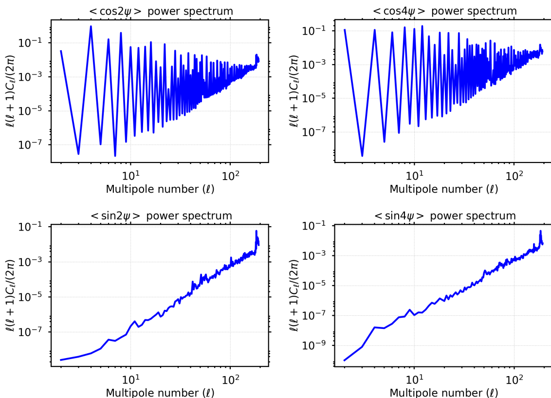
Figure 15. Crossing moment map power spectra. We show the power spectra of the maps of figure 14. The spectra of the two cosine maps, because of the azimuthally symmetric large power coherent on large scales shown in figure 2, have power spectra scaling similar to \ell^{-2} for the even moments, whereas the two sine maps (bottom) row exhibit spectra resembling pure white noise.
