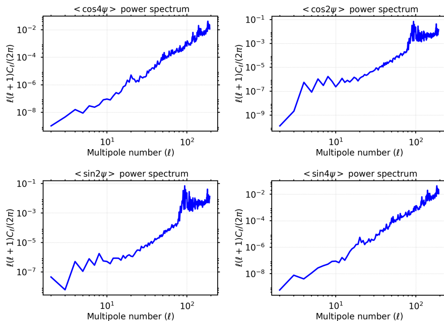
Figure 17. Crossing moment map power spectra (with rotating HWP). We show the power spectra for the maps in figure 16. The power spectra of the \langle \cos 2\psi \rangle and \langle \cos 4\psi \rangle have a white noise-like spectrum rather than an (\ell^{-2}) -like spectrum because the HWP has scrambled azimuthally symmetric component coherent on large-scale present in the case with no HWP.
