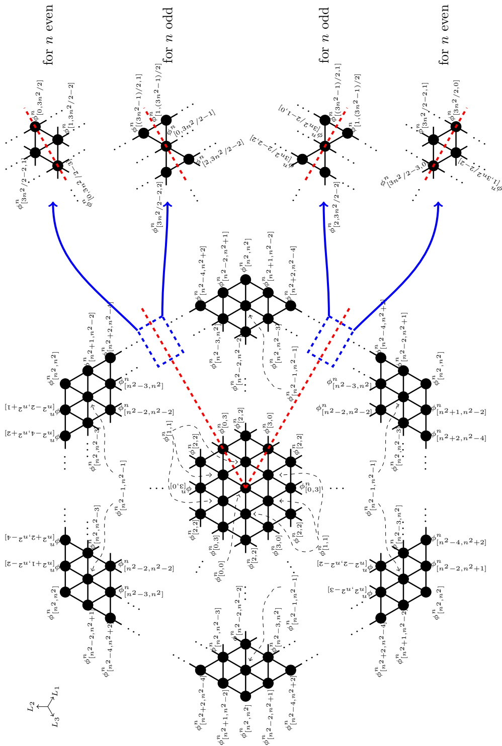
Figure 2. Representation of Z_{3,1}^{\text{line}}(\tau, m = n\epsilon, t_{f_1}, t_{f_2}, \epsilon, -\epsilon) on the weight lattice of \mathfrak{a}_2 .
