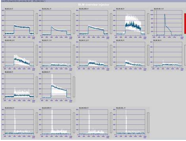
Figure 4: Display of the beam loss monitors during beam operation. Most of the monitors show the continuous dark current background, one BLM.49 produces an alarm (indicated in red). The BLMs in the dump line (bottom row) show in white color history data from previous trains.
