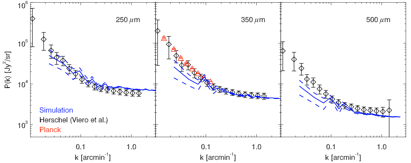
Fig. 13. Power spectrum of cosmic infrared background anisotropies at 250, 350, and 500 \mu\text{m} . The blue solid lines are CIB anisotropies measured in our simulation and 1\sigma confidence regions are represented by the dashed lines. The black diamonds and the red triangles are the measurements of Viero et al. (2013b) and Planck Collaboration XXX (2014), respectively.
