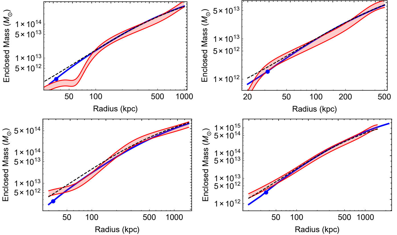
Fig. 7. Same as Fig. 6 for the NFW normal phase. Only the case of \Lambda m^3 = 0.3 \times 10^{-3} \text{ eV}^4/c^8 is shown. r_s for each cluster is defined as a fraction 1/n of the virial radius, where n is 5, 6, 4, and 4 for clusters A133, A262, A468, and A1413, respectively. The NFW normal phase follows the \Lambda CDM prediction much more closely than the isothermal normal-phase model. Central regions are still consistently smaller than in the \Lambda CDM predictions, which needs to be investigated in further work.
