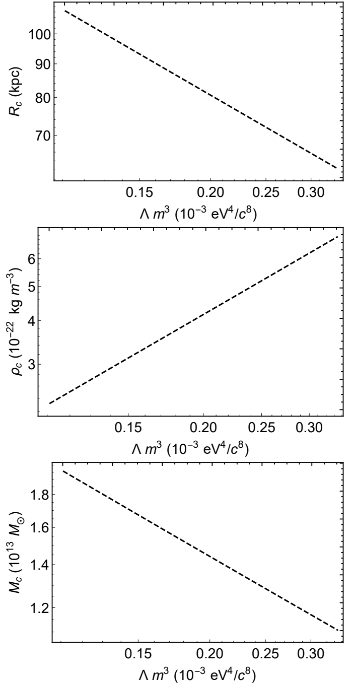
Fig. 2. Change in core radius ( top panel ), density at core radius ( middle panel ), and core mass ( bottom panel ) as a result of different values of \Lambda m^3 . This is a visual representation of the relationships listed in Eq. (19).
