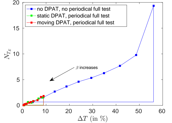
(b) Trade-off between test escape and test time savings achieved by different adaptive test flows.
