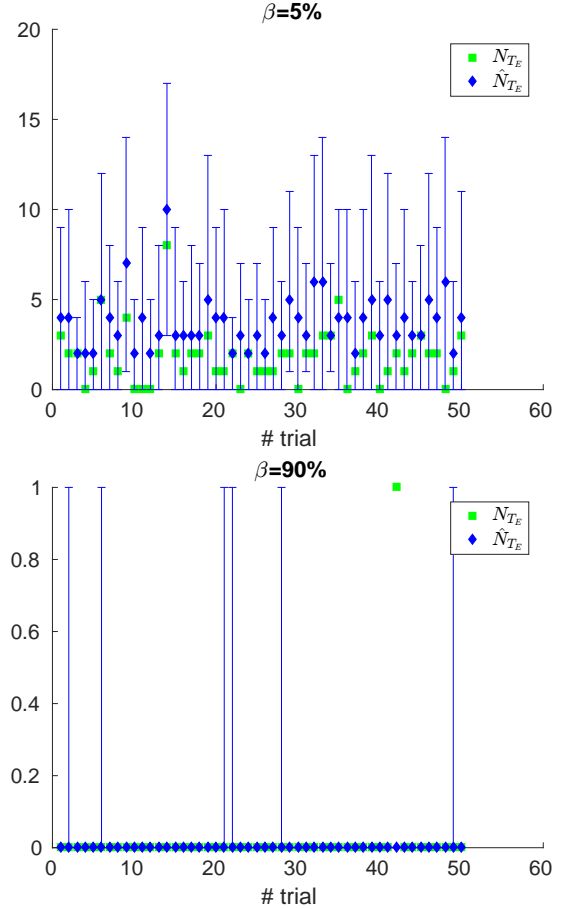
Fig. 10: True and estimated absolute test escape across the 50 trials for two “extreme” values of \beta , showing also the 95% confidence interval.
