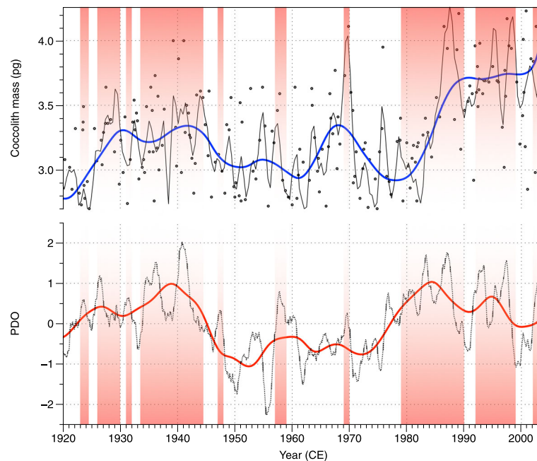
Fig. 5 Comparison between the mass of coccoliths of E. huxleyi , G. ericsonii , and G. muellerae (Top) and Pacific Decadal Oscillation (PDO) index (Mantua and Hare 2002). Red bands highlight periods of high PDO
