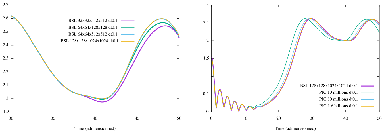
Figure 19: Time evolution of electric energy, with convergence of BSL (left) and PIC (right). A = 0.1 , second test case. Different grid sizes for BSL and different numbers of particle for PIC are used. Time step is \Delta t = 0.1 . The reference solution is here BSL with grid size 128 \times 128 \times 1024 \times 1024 .
