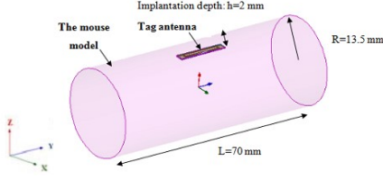
Fig. 2. Implanted tag in the homogenous body phantom.
