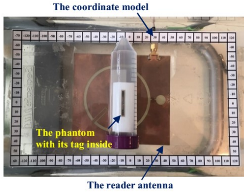
Fig. 5. Antenna reader with its system of coordinates and the phantom with its tag inside.
