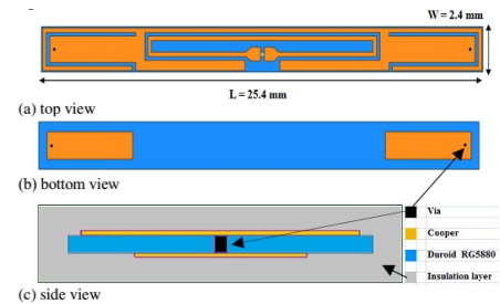
Fig. 1. Geometry of the antenna.
