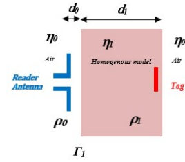
Fig. 4. Transmission and reflection on the dielectric layer.
