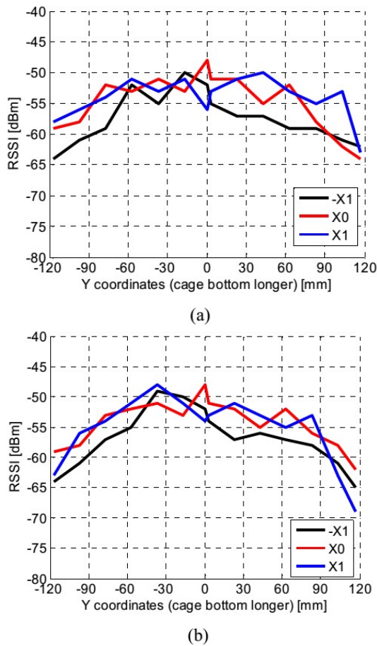
Fig. 9. RSSI measured values at 868 MHz when the phantom model is oriented along the X axis (a), Y axis (b) and moves along the Y axis.
