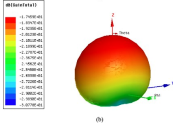
Fig. 3. (a) reflection coefficient and (b) simulated radiation pattern of the implanted antenna.
