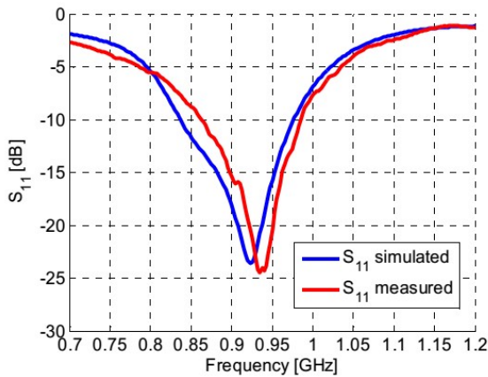
Fig. 6. Simulated and measured S_{11} parameter for the reader antenna.
