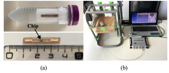
Fig. 7. (a) antenna prototype in the phantom model, (b) measurement set-up.
