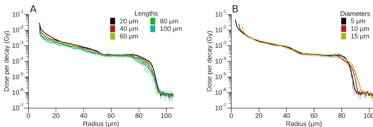
Figure 5. Dose per event (Gy) for ^{212}\text{Pb} . (A) Variation of absorbed dose (Gy) for a 15 \mu\text{m} diameter vessel as a function of vessel length. (B) Variation of absorbed dose (Gy) for a vessel of length 40 \mu\text{m} as a function of vessel diameter.
