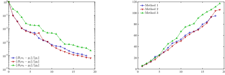
Figure 5: Test case 2. Left: relative residual at each iteration of the greedy algorithm. Right: cumulated number of alternating minimization iterations in the greedy algorithm.
