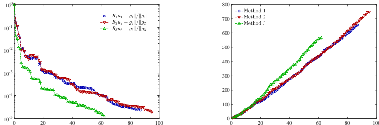
Figure 9: Test case 3. Left: relative residual at each iteration of the greedy algorithm. Right: cumulated number of alternating minimization iterations in the greedy algorithm.
