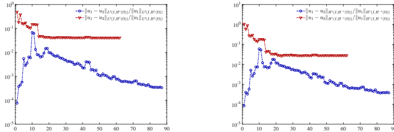
Figure 11: Test case 3: comparison of the solutions produced by Methods 1, 2, 3 in two norms: L^2(I; H^1(\Omega)) (left) and H^1(I; H^{-1}(\Omega)) (right).
