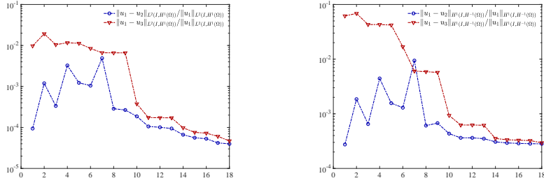
Figure 7: Test case 2: comparison of the solutions produced by Methods 1, 2, 3 in two norms: L^2(I; H^1(\Omega)) (left) and H^1(I; H^{-1}(\Omega)) (right).
