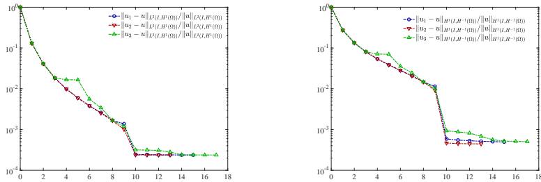
Figure 3: Test case 1: comparison of the errors produced by Methods 1, 2, 3 in two norms: L^2(I; H^1(\Omega)) (left) and H^1(I; H^{-1}(\Omega)) (right).
