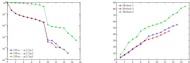
Figure 1: Test case 1. Left: relative residual at each iteration of the greedy algorithm. Right: cumulated number of alternating minimization iterations in the greedy algorithm.
