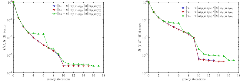
Figure 3: Test case 1: comparison of the errors produced by Methods 1, 2, 3 in two norms: L^2(I; H^1(\Omega)) (left) and H^1(I; H^{-1}(\Omega)) (right); in both cases, the curves for Methods 1 and 2 almost overlap.
