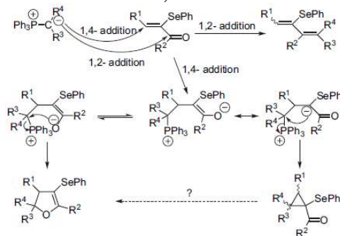
Scheme 6. Mechanistic considerations.
