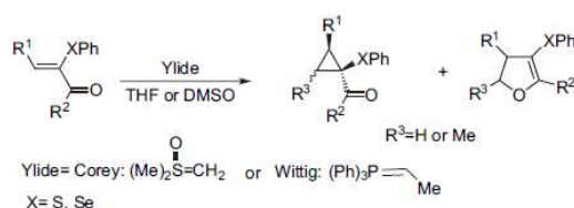
Scheme 7. Influence of the ylide on the cyclopropane/dihydrofuran ratio.
