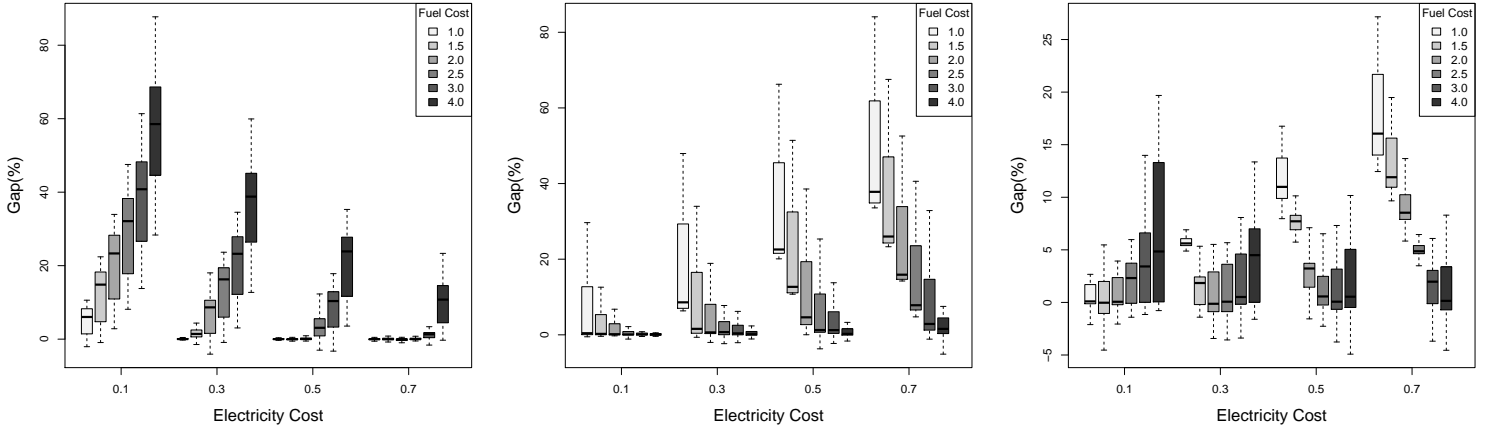
Figure 6.1: Gap(%) of the solutions obtained with an homogeneous fleet of ICEV (left), BEV (middle), and PHEV (right), relative to the optimized solution with a mixed fleet.
