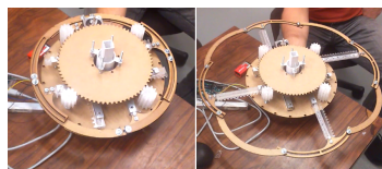
(b) IrregularRing-4arms-8arcs
