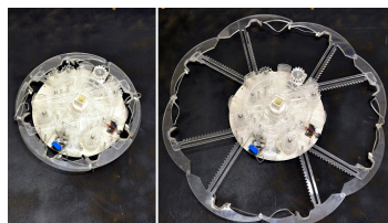
(c) RingLike-8arms-8arcs
