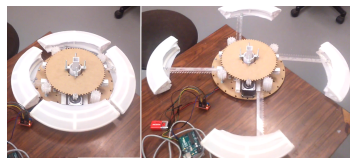
(a) DiscontinuousRing-4arms-4arcs
