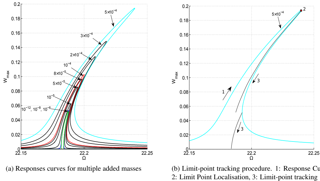
Figure 2: Response curves of the central resonator for a varying non-dimensional added mass.
