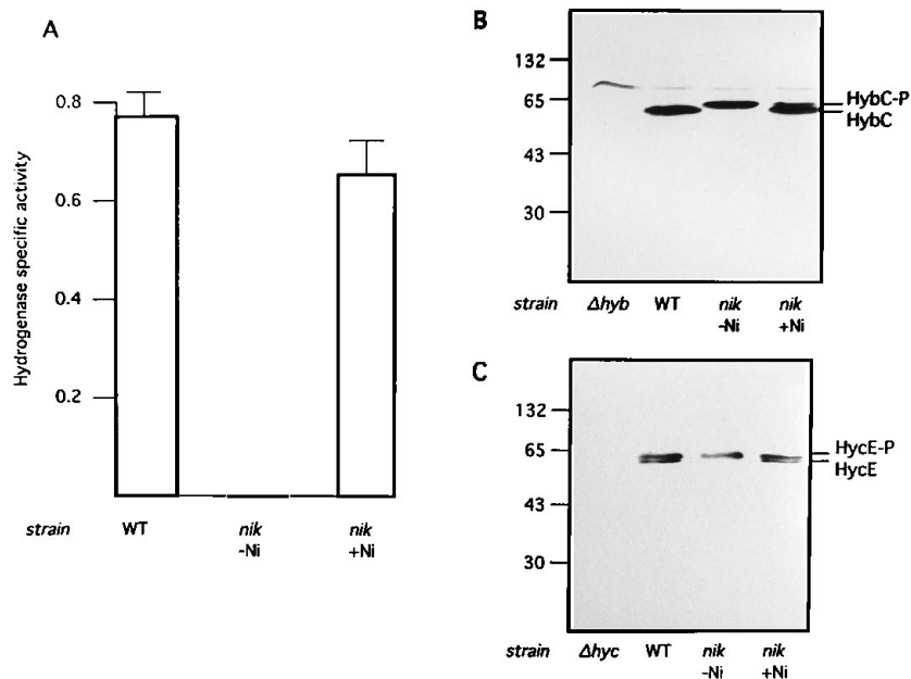
FIG. 2. Nickel-dependent restoration of hydrogenase activity and large subunit processing in the nik mutant. Wild-type B178 (WT) and its derivatives NB01 ( nik ), HYD720K ( \Delta hyb Δnik ; this strain is described as \Delta hyb in panel B), and HD700 ( \Delta hyc) were grown anaerobically at 37°C in LB medium. As noted, 300 \mu M NiCl 2 was added to cultures ( \Delta nik + Ni) after 3 h of incubation (OD 600 = 0.3). After 1 h of additional incubation, cells were harvested. Under these conditions, the processing of the precursor of HybC is not completed, which allows a clear distinction between the precursor and the processed form. For other cultures grown in the absence of nickel (-Ni) (WT, \Delta hyb, \Delta hyc, and Δnik -Ni), cells were harvested after a total of 4 h of incubation. The hydrogenase specific activity (A) was measured as described in Materials and Methods. The cellular contents of the precursors and processed forms of the large subunits of HYD2 (HybC-P and HybC, respectively) (B) and HYD3 (HycE-P and HycE, respectively) (C) were detected by immunoblotting after the separation of proteins (20 \mu g for each sample) by SDS-12.5% PAGE. For each culture, the same sample was used to perform the three experiments. Strains HYD720K ( \Delta hyb Δnik ) and HD700 ( \Delta hyc) were used here to verify the identities of HybC and HycE, respectively.
