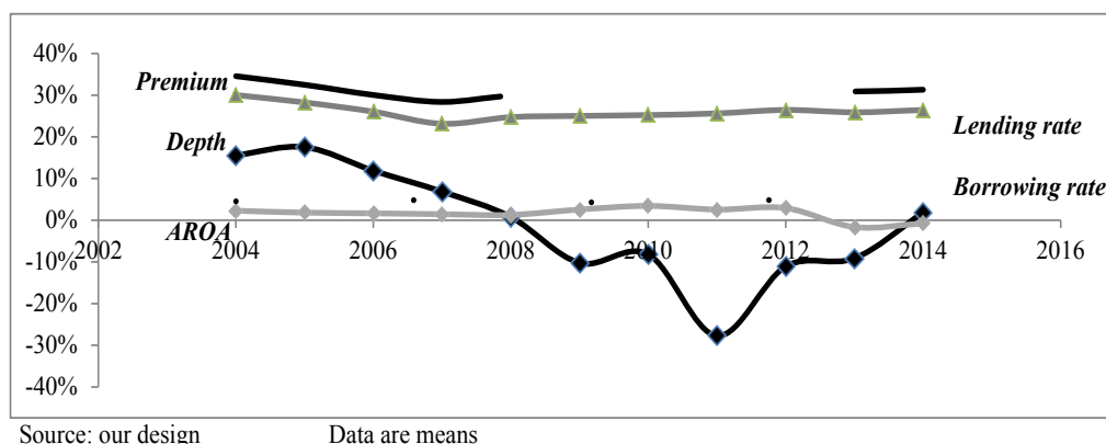
Figure 1: The trend of lending and borrowing rates, Premium, AROA and Depth.
