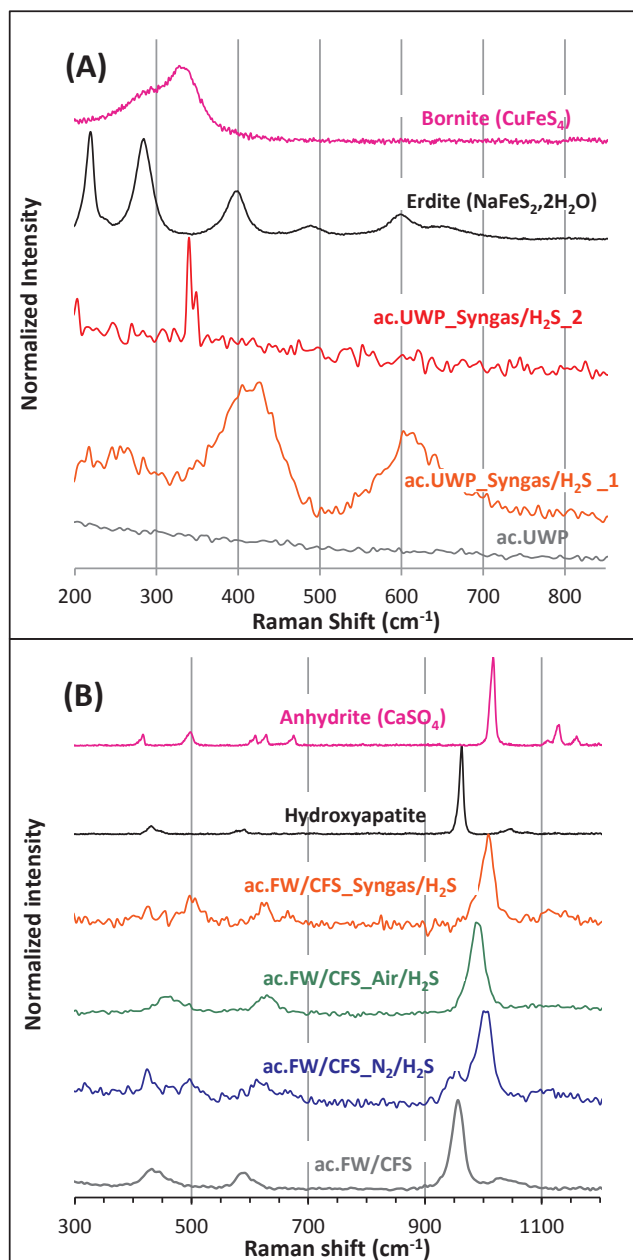
Fig. 4. Normalized Raman spectra of (A) ac.UWP, and (B) ac.FW/CFS before and after the \text{H}_2\text{S} removal tests. Experimental spectra were compared with the RRUFF database spectra in order to identify the sulfur species formed.
